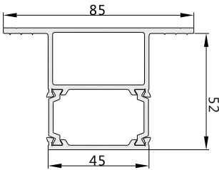
GJ6050A-1 (Drawing)
