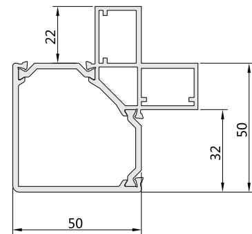
PA4028三通 (Corner)
