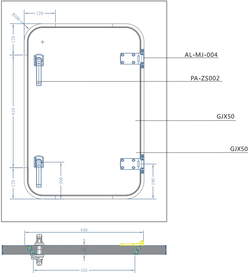
GJ-R50检修门(R50见光) (GJX50-R Access Door(R50 Lighted part )
