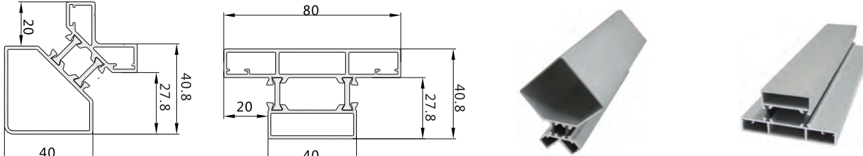
GJ4028G (Drawing)
