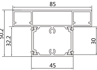
GJ6050M-1 (Drawing)
