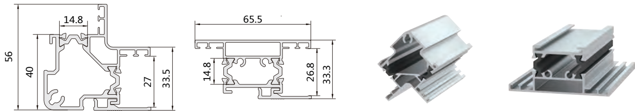
GJ4225 ( 实物图 ) GJ4225-1 ( 实物图 ) (Frame Profile) (Omega Profile)
