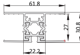
GJ4027M-1 (Drawing)
