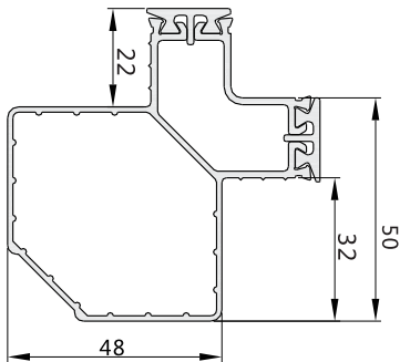
PA5075三通 (Corner)
