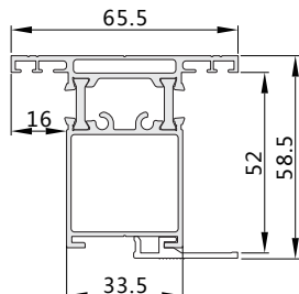
GJ6750-1 (Drawing)
