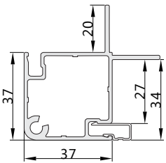
GJ3727 (Drawing)
