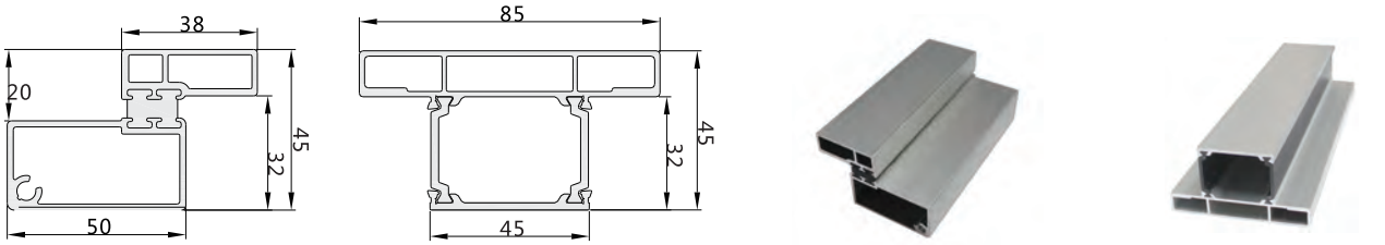
GJ5045G (Drawing)
