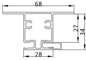
GJ3727-1 (Drawing)
