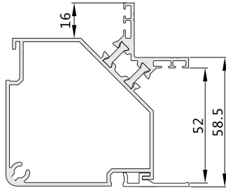
GJ6750 (Drawing)
