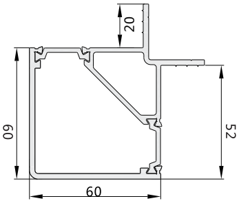
GJ6050A (Drawing)
