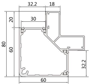
GJ6050M (Drawing)
