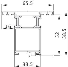
GJ6752-1 (Drawing)
