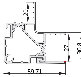
GJ4027M (Drawing)
