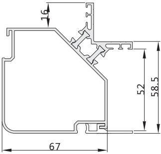
GJ6752 (Drawing)
